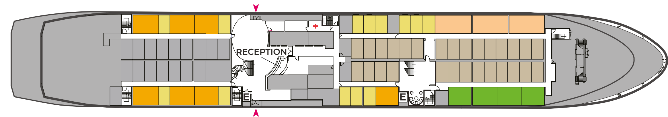
DECK 4
